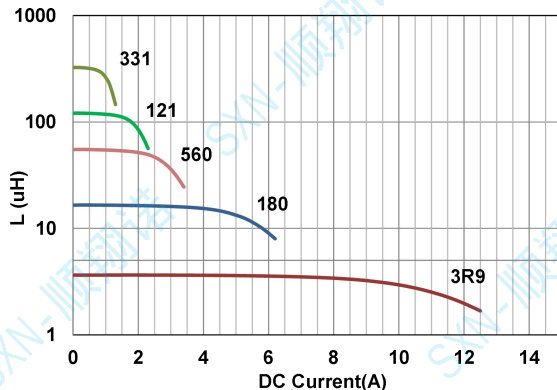
Inductance vs DC Current Curve
