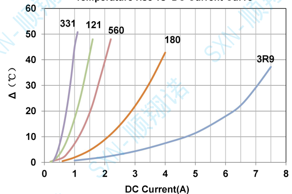
Temperature rise vs DC Current Curve
