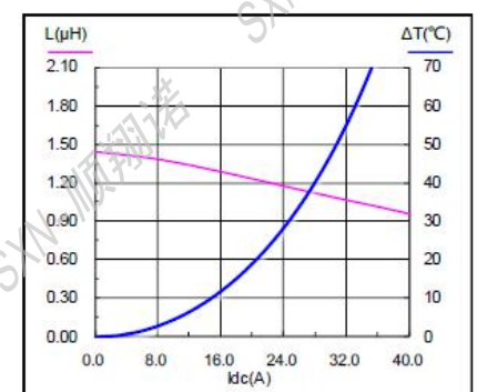
SMMS1350-1R5M
