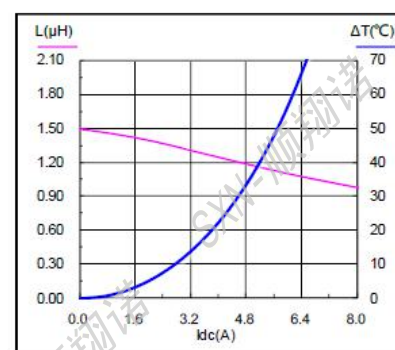
SMMS0520-1R5M
