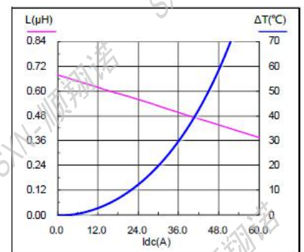
SMMS1350-1R5M
