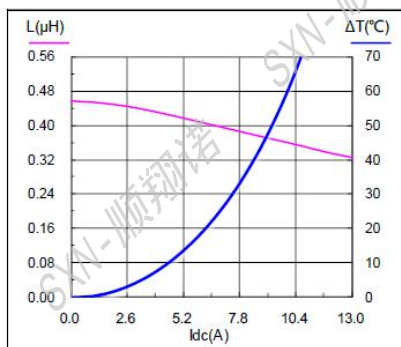
SMMS0420-R47M
