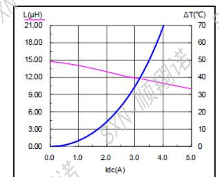
SMMS0630-150M
