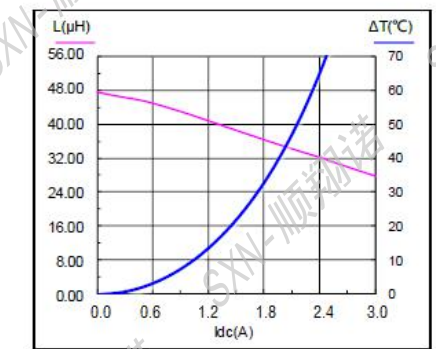
SMMS0630-470M
