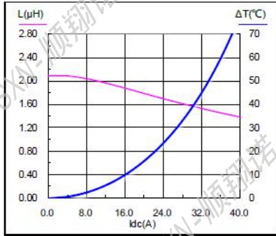
SMMS1770-100M
