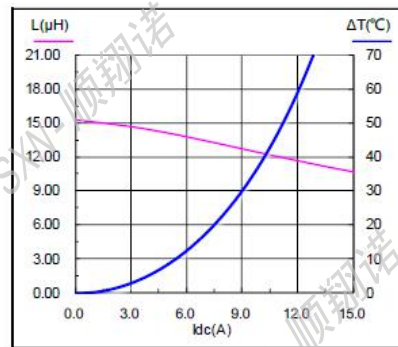
SMMS1770-470M
