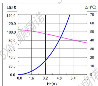
SMMS1770-101M
