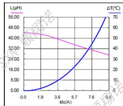
SMMS1770-470M
