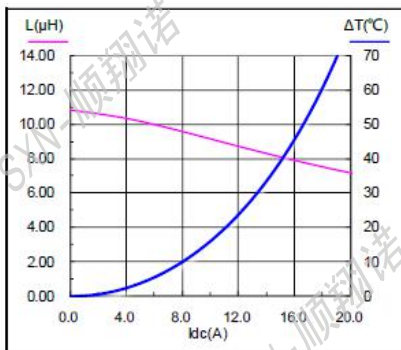
SMMS1770-330M
