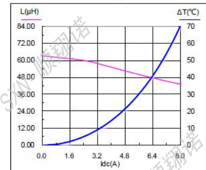
SMMS1770-680M
